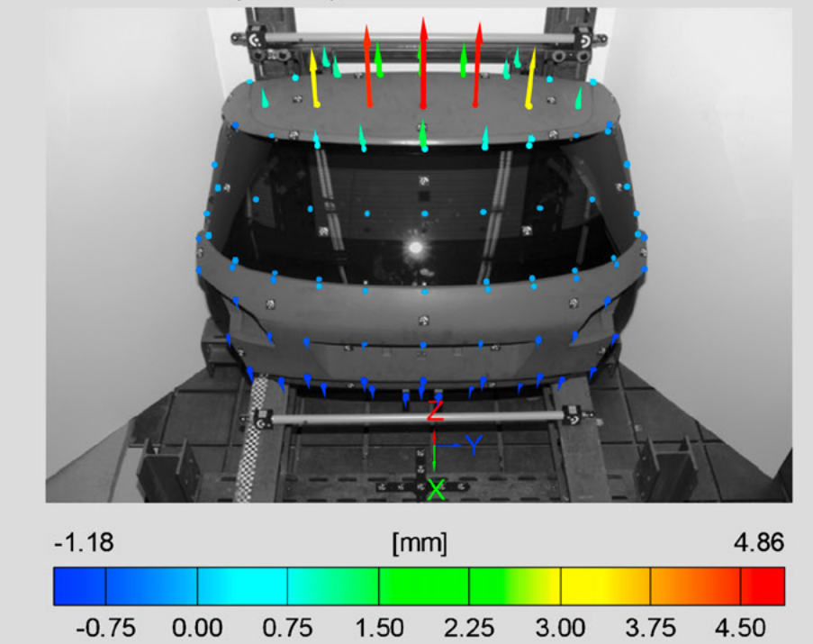
Deformation (Z-Axis)
