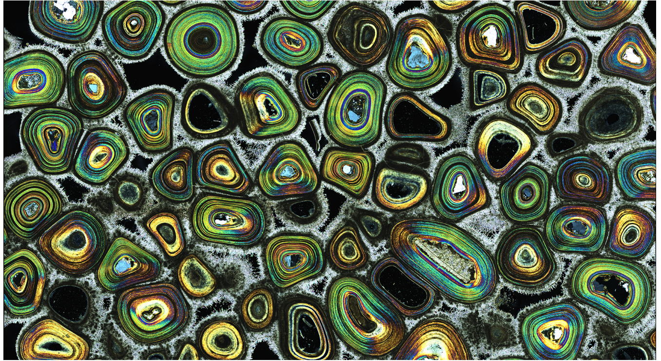
Thin section of Karlsbader Sprudelstein, scanned with 10x N-Achroplan 045 Pol. A merged image of the cross linear polarized light channels is shown. Sample courtesy of Bernardo Cesare, Università di Padova, Italy
