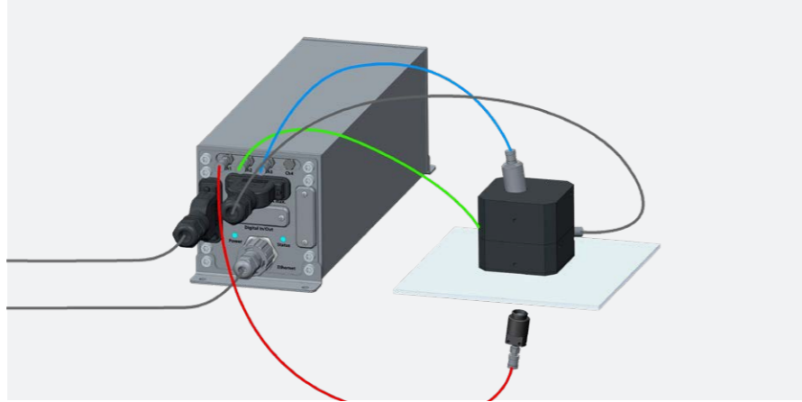
Reflection and transmission measurement with bypass
